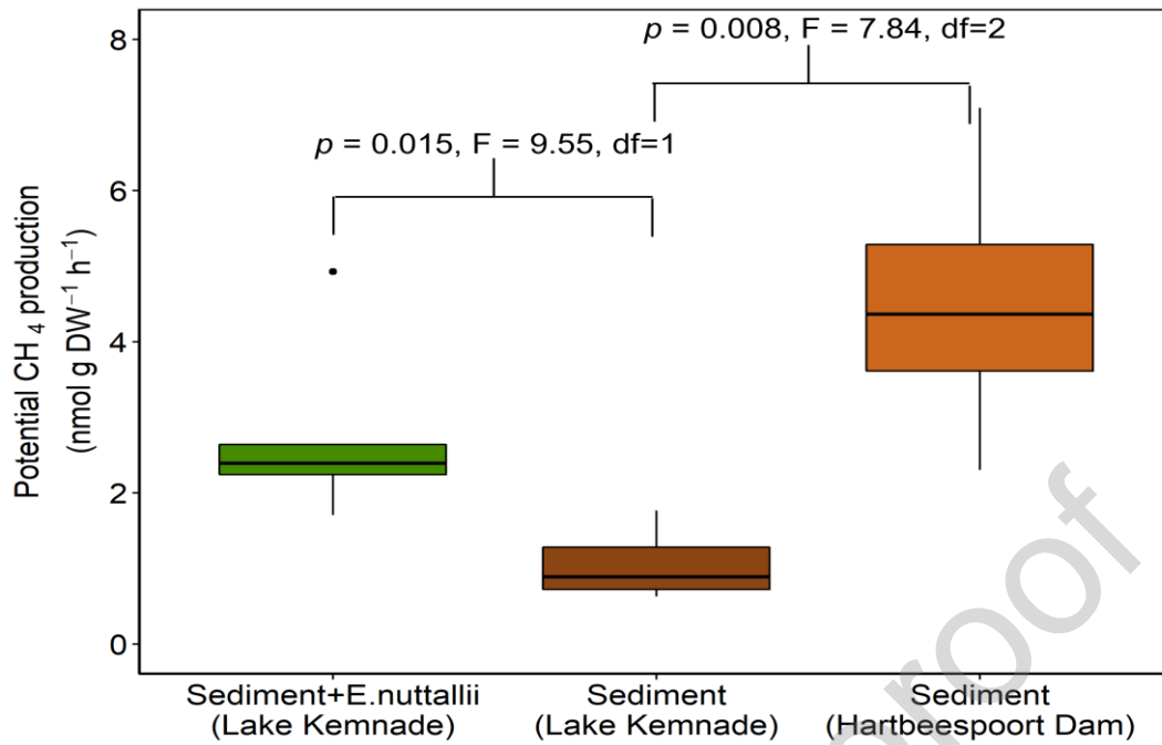
Fig 5. Potential hourly methane production, derived from incubations of sediment with (left) or without (middle) E. nuttallii at Lake Kemnade, and sediment at Hartbeespoort Dam (right).
